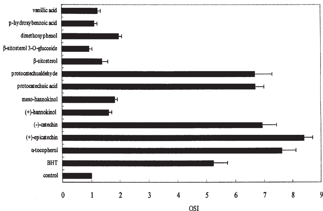
FIG. 1. Antioxidant activity of the compounds isolated from Amomum tsao-ko based on the oxidative stability index (OSI) (90°C, 1 \mu mol/5 g oil).
